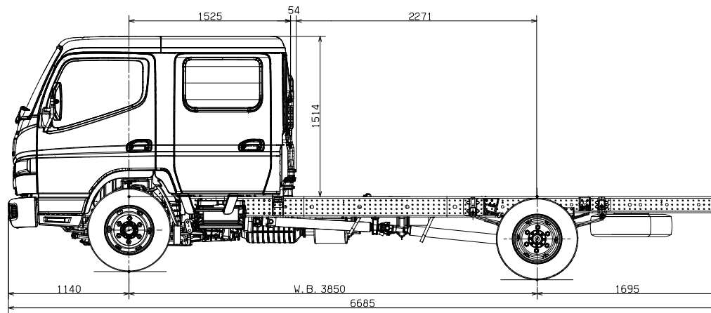
CANTER 816 CREW CAB – 'G' WHEELBASE
