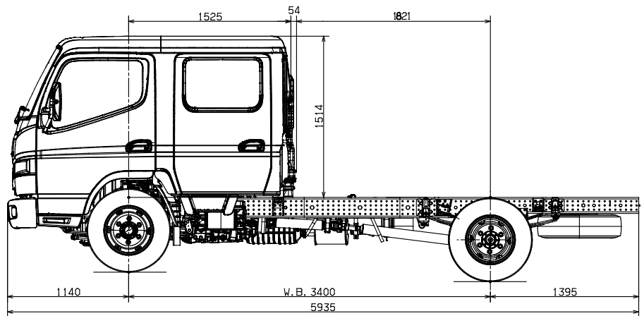
CANTER 816 CREW CAB – 'E' WHEELBASE
