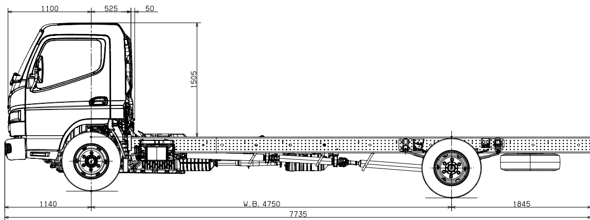
CANTER 918 CREW CAB – ‘K’ WHEELBASE
